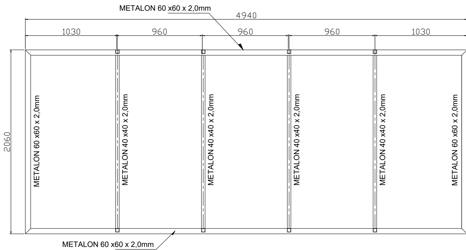
VISTA FRONTAL
